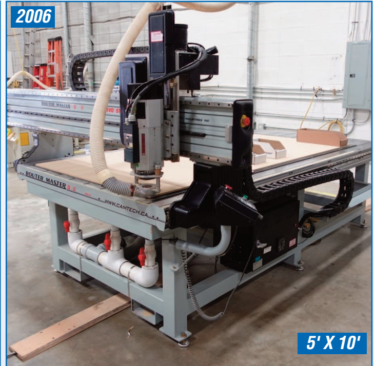
CAM TECH ROUTER MASTER II 52, CNC ROUTER
